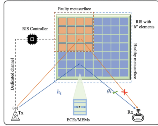
Figure 2. Inaccurate reflections from a faulty RIS element may lead to communication disruption.
