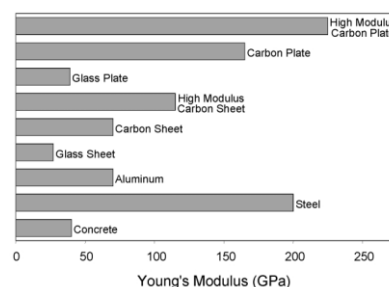
Figure 1. Elastic (Young 's) modulus [1]
