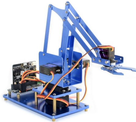
Figure 3. Robot arm
