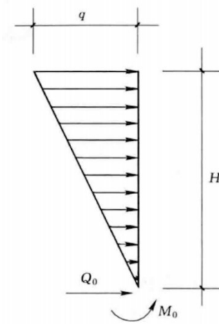
Figure 3. Force diagram
