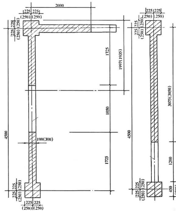
Figure 2. drawing of the shear wall
