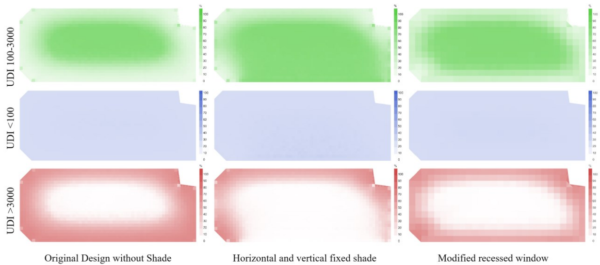
Figure 4: UDI Diagram for different shading devices
