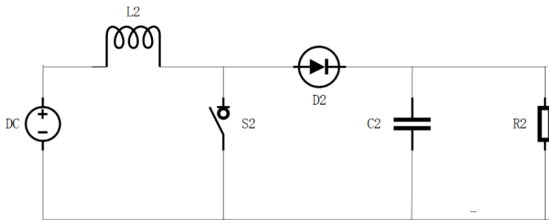
Figure 2: DC-DC boost converter.
