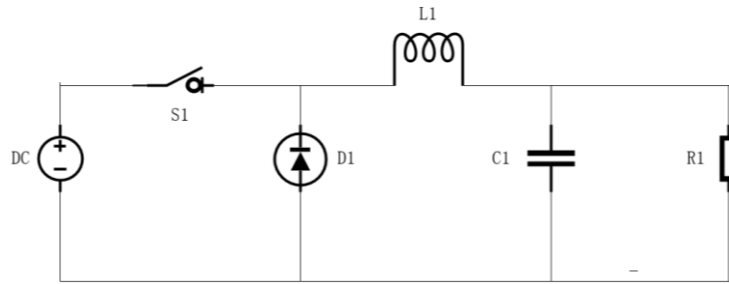
Figure 1: DC-DC buck converter.
