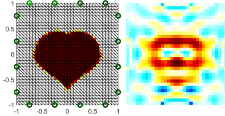
Figure 3: Photoconductivity simulation result using the TSVD method.
