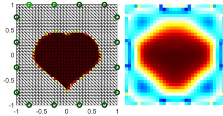
Figure 2: Photoconductivity simulation result using the Kalman filter method.
