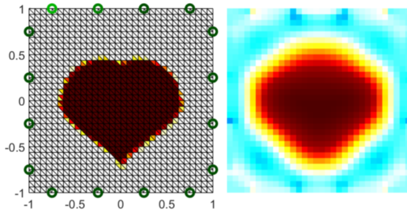
Figure 1: Photoconductivity simulation result using the Gauss-Newton method.
