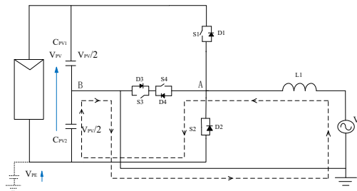
Figure 15: AC power supply negative half fundamental period operating mode 1
