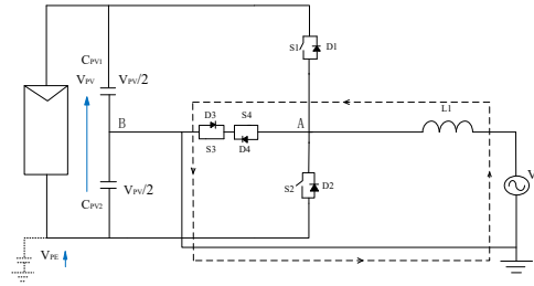
Figure 16: AC power supply negative half fundamental period operating mode 2
