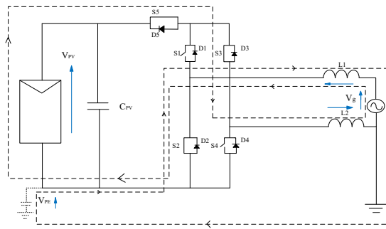
Figure 3: AC power supply negative half fundamental period operating mode 1
