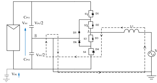
Figure 11: AC power supply negative half fundamental period operating mode 1
