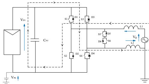
Figure 7: AC power supply negative half fundamental period operating mode 1
