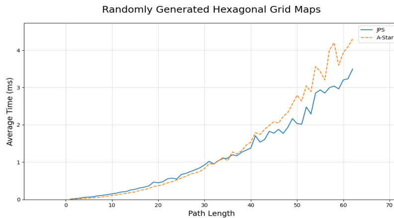
Figure 4: Result of the experiment with rounds 50, times per round 100 and obstacle rate 0.25.
