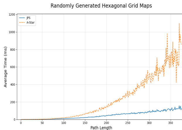
Figure 3: Result of the first experiment with rounds 300, times per round 50 and obstacle rate 0.25.
