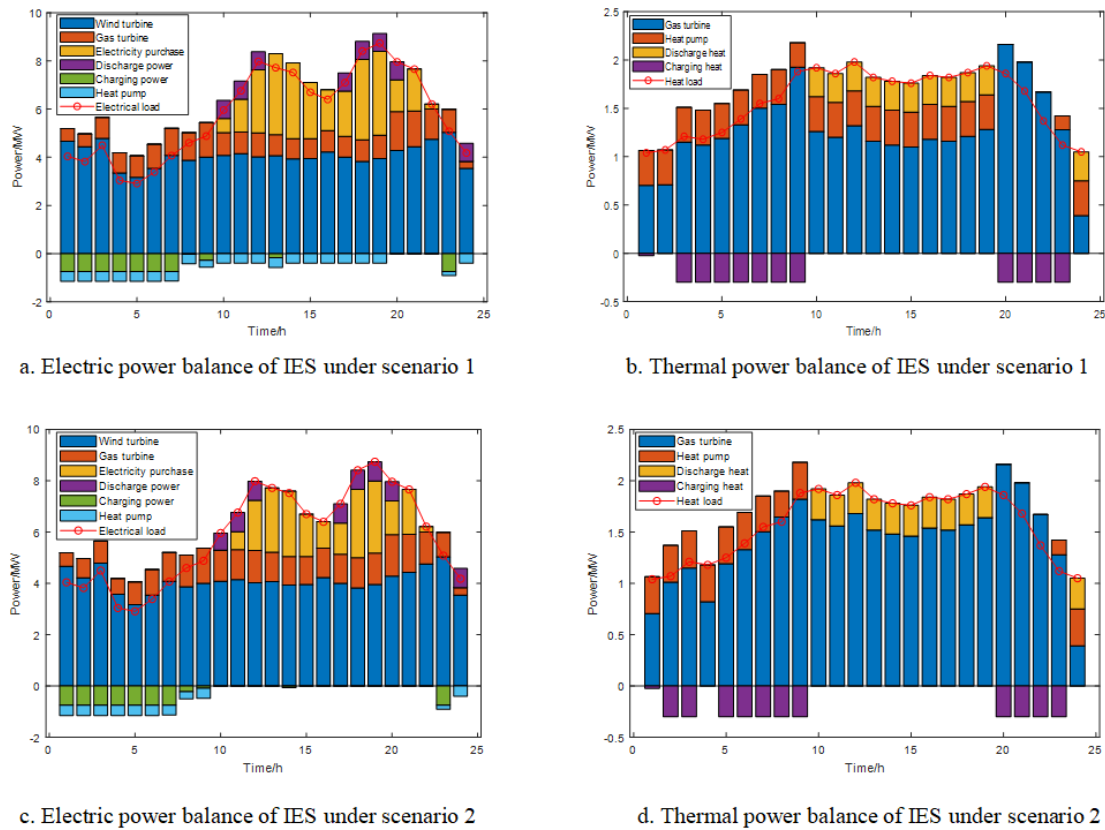
Figure 4: Electrical/thermal power balance of IES in different scenarios
