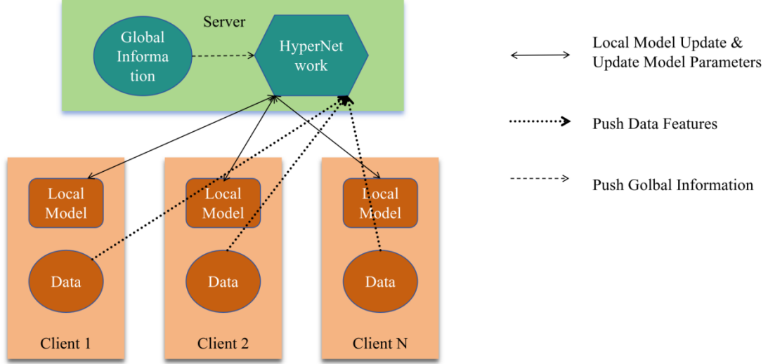
Figure 2: Illustration of pFedHN mechanism (picture credit: original)
