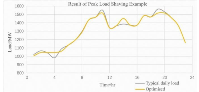
Figure 2: EV aggregation charging/discharging result
