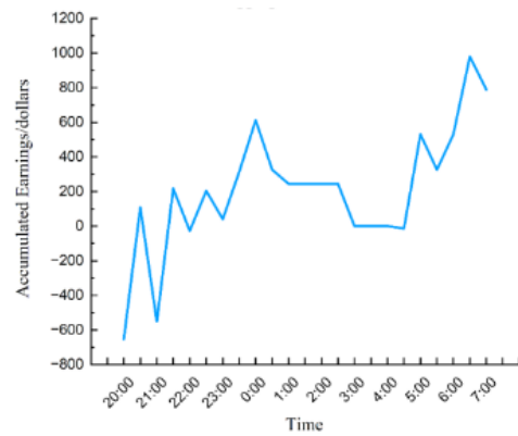
Figure 4: EV aggregator average power profit
