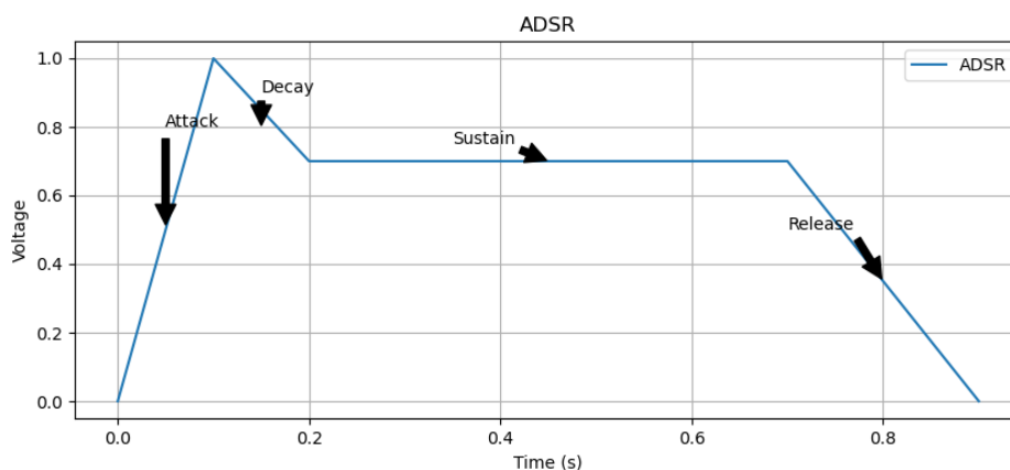
Figure 2: Envelope generators full cycle (photo/picture credit: original)
