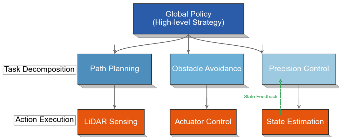
Figure 2: Hierarchical reinforcement learning framework diagram [6]
