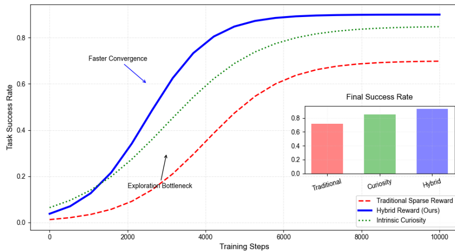
Figure 3: Comparison of sparse reward optimization techniques [10]
