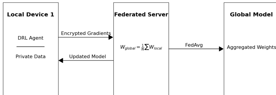
Figure 4: Privacy protection architecture for federated learning and DRL[12]
