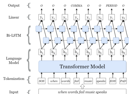
Figure 2: RoBERTa-BiLSTM Model architecture [11]
