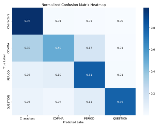
Figure 3: Normalized confusion matrix on validation set
