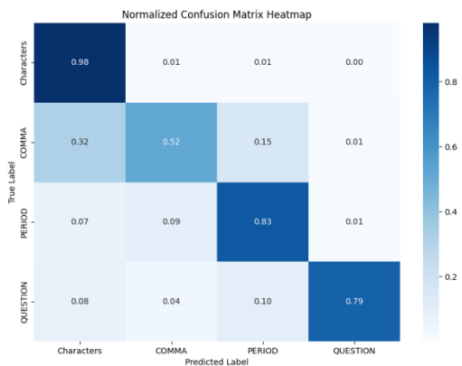
Figure 4: Normalized confusion matrix on test set
