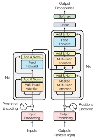
Figure 1: The Transformer Model architecture [12]
