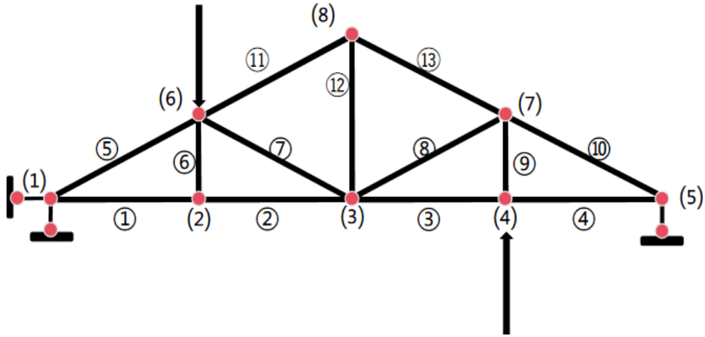
Figure 5: Shear load application schematic
