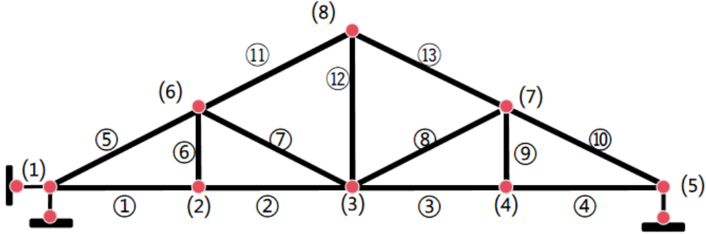
Figure 1: Truss schematic diagram
