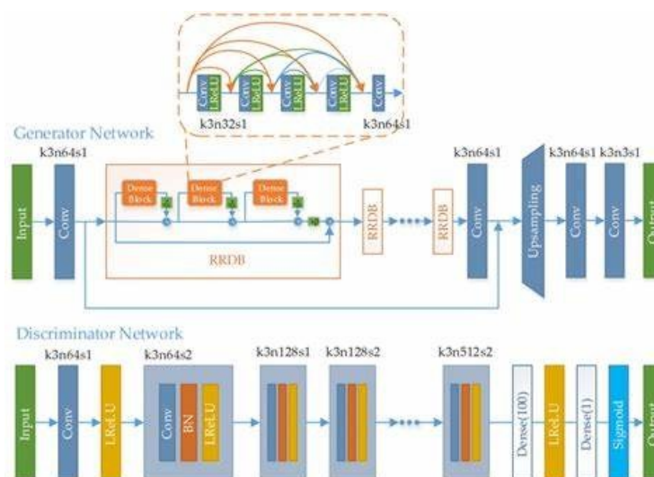
Figure 1: GAN network architecture with generator and discriminator modules (source: researchgate.net)
