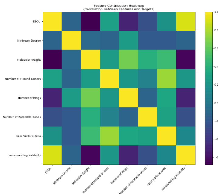
Figure 2. Feature contribution heatmap
