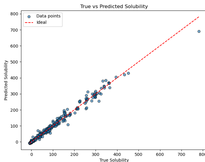
Figure 3. True vs. predicted solubility scatter plot
