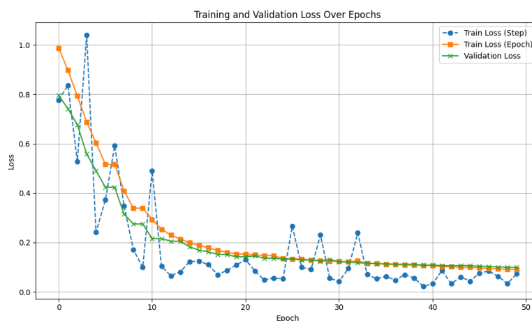
Figure 1. Training and validation loss over epochs
