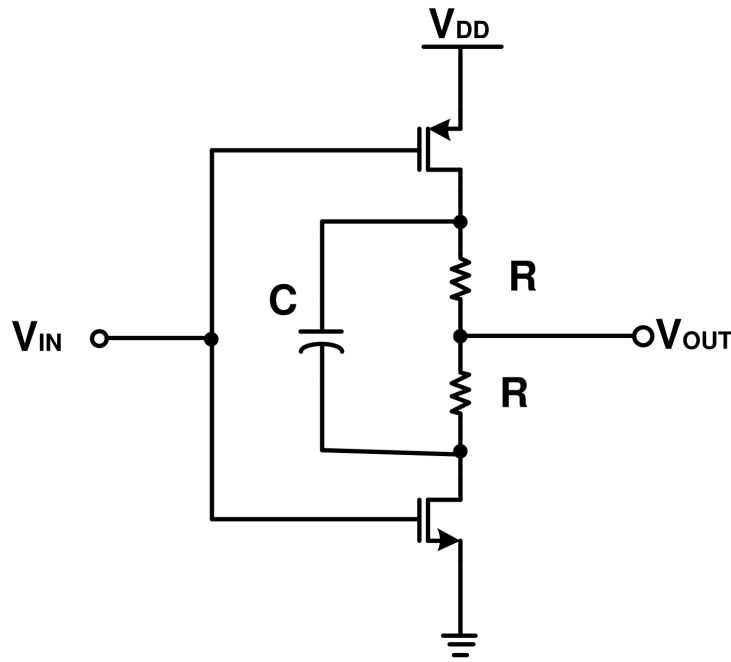
Figure 2: Low-noise inverter amplifier
