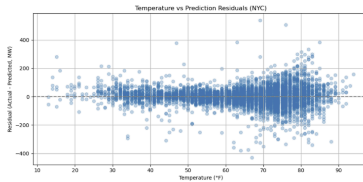
Figure 2. Temperature vs. prediction residuals (NYC)
