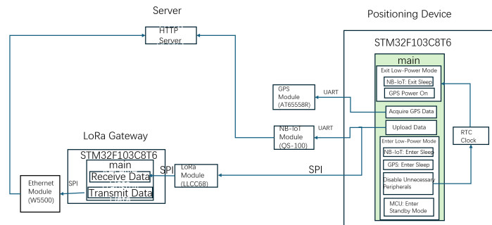
Figure 2. Terminal–LoRa gateway–server topology with NB-IoT primary, LoRa fallback
