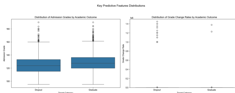
Figure 3. Key predictive features distributions
