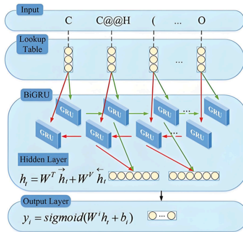
Figure 3. The network structure of BIGRU
