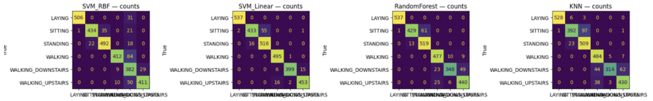
Figure 1. Performance of SVM RBF, SVM Linear, Random Forest, and KNN
