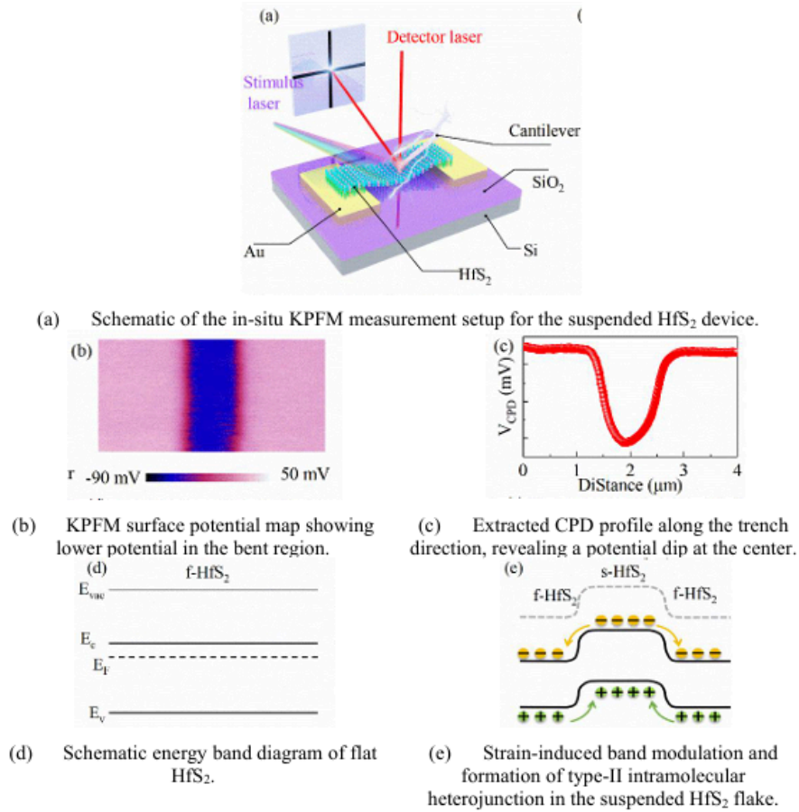
Figure 2. In-situ KPFM characterization of suspended \text{HfS}_2 flake
