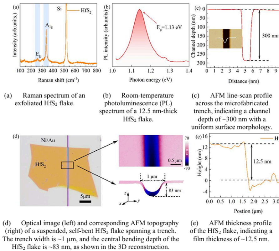
Figure 1. Structural and morphological characterization of \text{HfS}_2 thin films and self-bent devices
