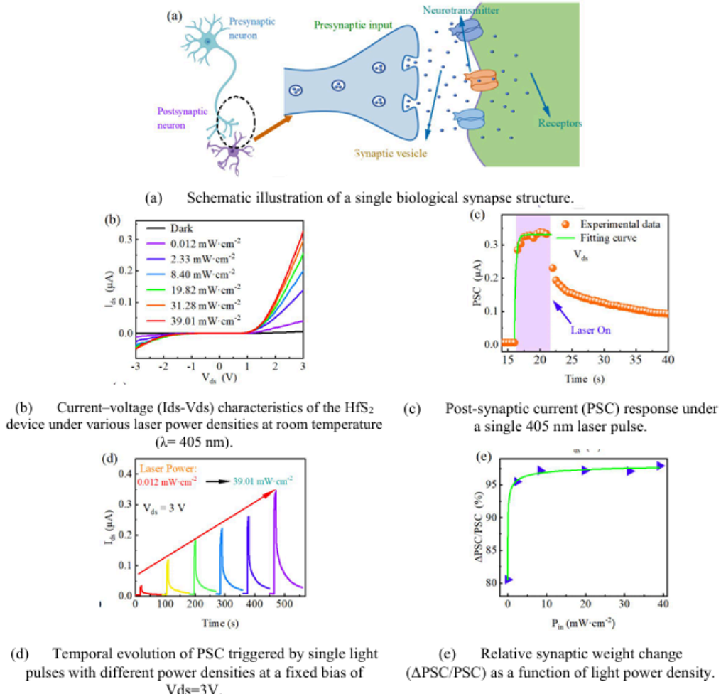
Figure 3. Optical synaptic responses of the bent \text{HfS}_2 device
