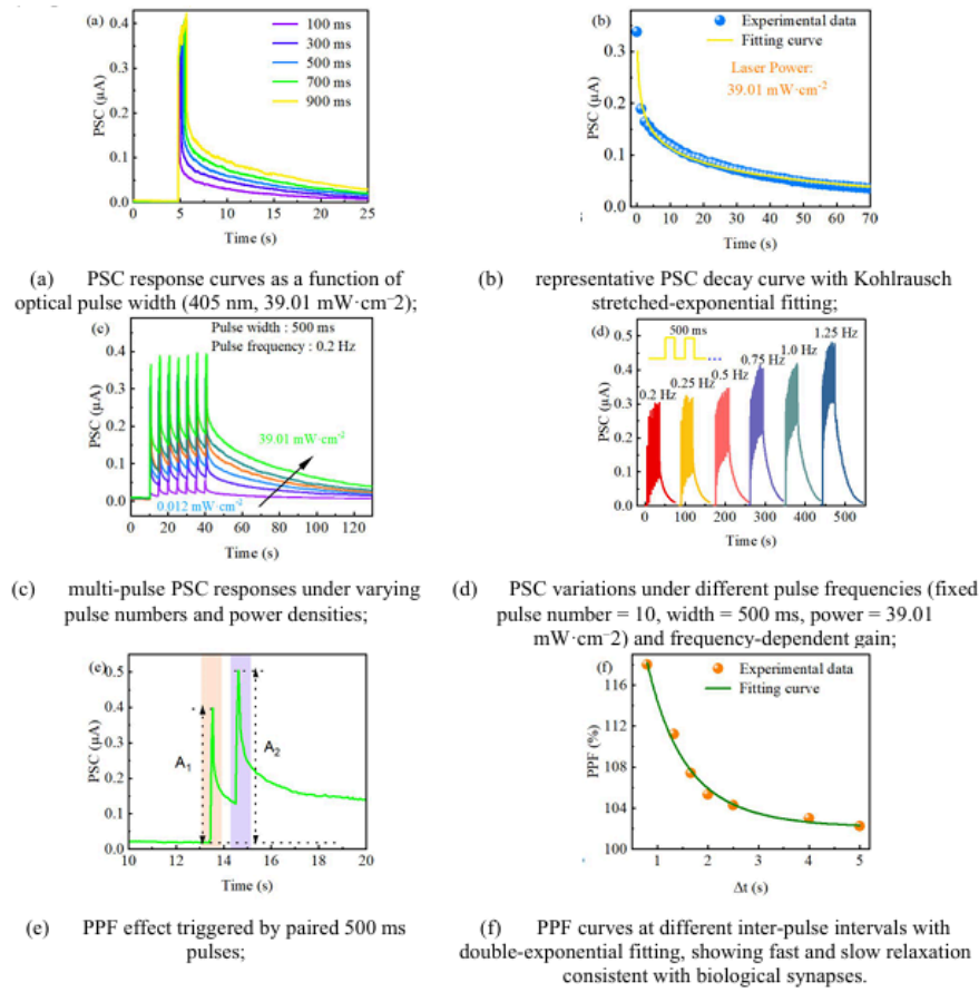
Figure 4. Synaptic plasticity under varied pulse parameters and paired-pulse facilitation
