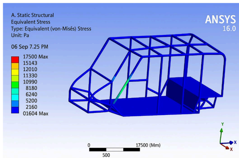
Figure 1. Static analysis model of the vehicle body structure
