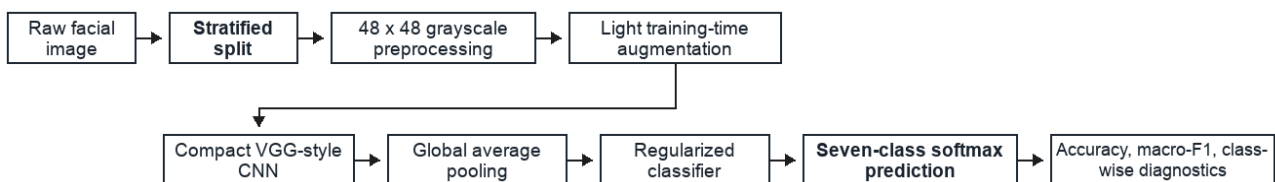
Figure 1. Stability-oriented workflow of the proposed small-sample FER framework. (picture credit: original)
