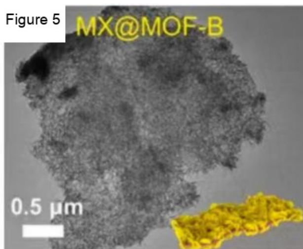
Figure 5. TEM morphology of the MX@MOF-B composite flame retardant
