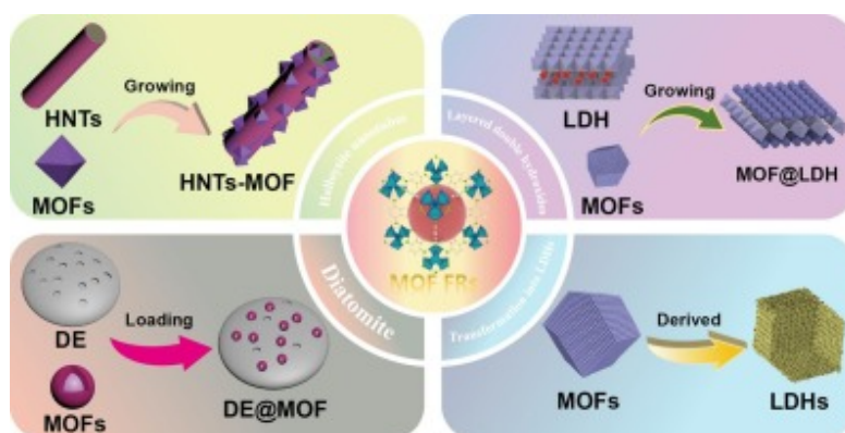
Figure 2. Synthesis routes for MOF-clay flame retardants: (a) halloysite nanotubes; (b) layered double hydroxide; (c) diatomite; (d) MOF-derived layered double hydroxide [5]
