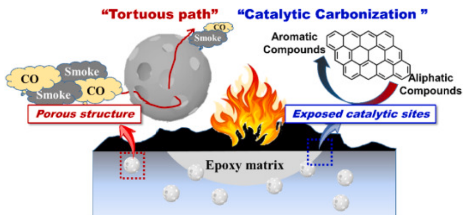
Figure 1. Proposed flame-retardant mechanism of an MOF-derived porous transition-metal oxide in epoxy resin (EP/C-ZrO 2 sample) [3]
