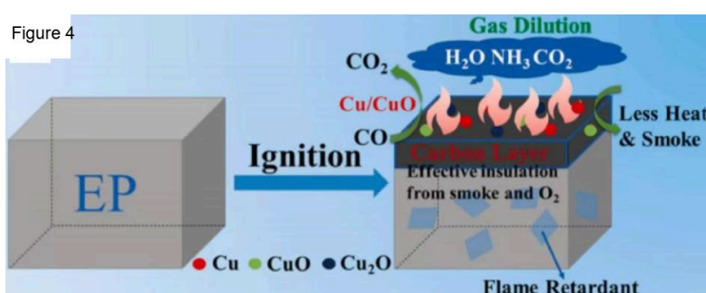
Figure 4. Schematic flame-retardant mechanism of a copper-based MOF in epoxy resin (EP)
