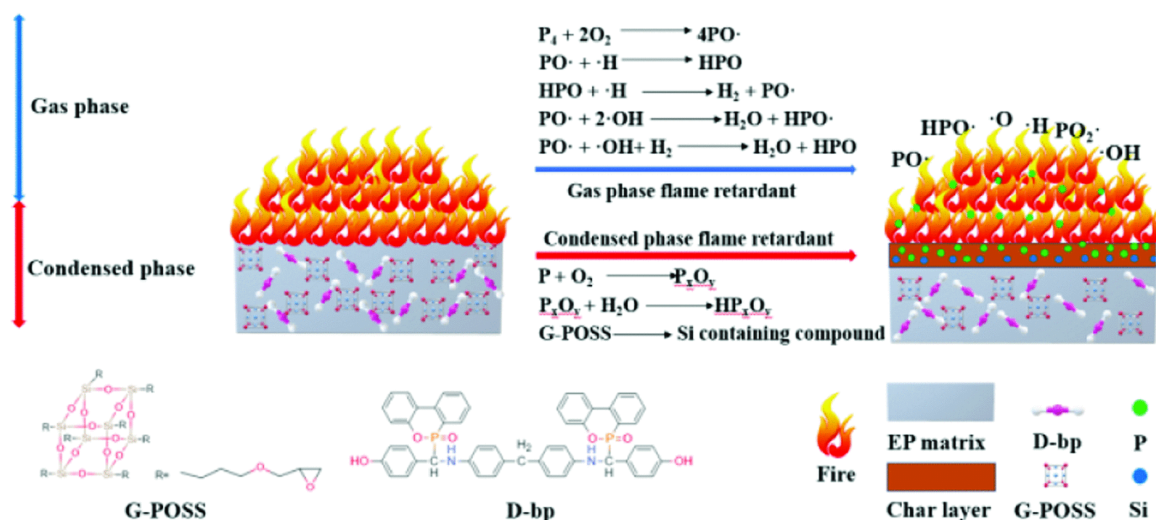
Figure 5. POSS/D-bp/DGEBA hybrid composites [25]
