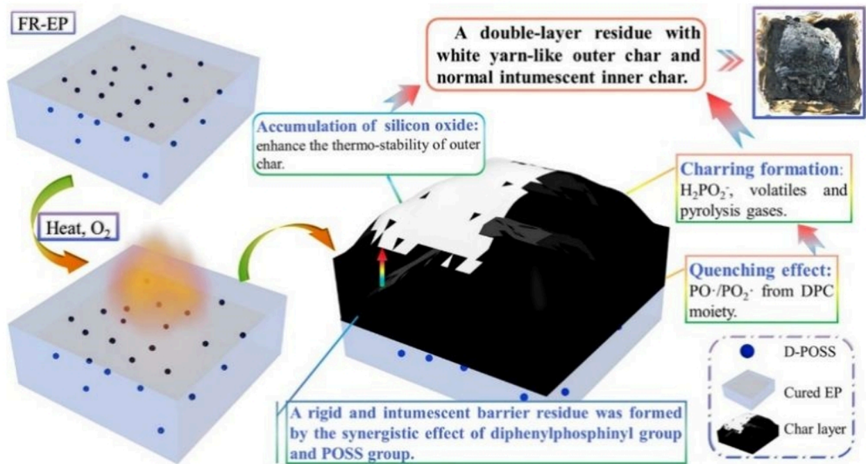
Figure 2. Illustration of the flame-retardant mechanism for the FR-EP [12]
