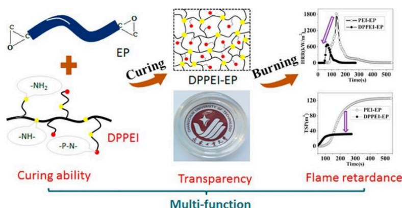
Figure 6. Synthesis and performance of multifunctional DPPEI-EP [26]
