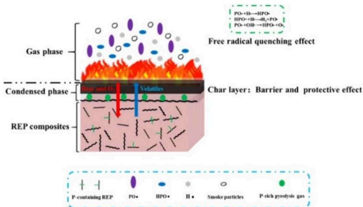
Figure 1. Schematic diagram of radical quenching effect [2]
