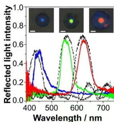
Figure 1. Reflectance spectrum
