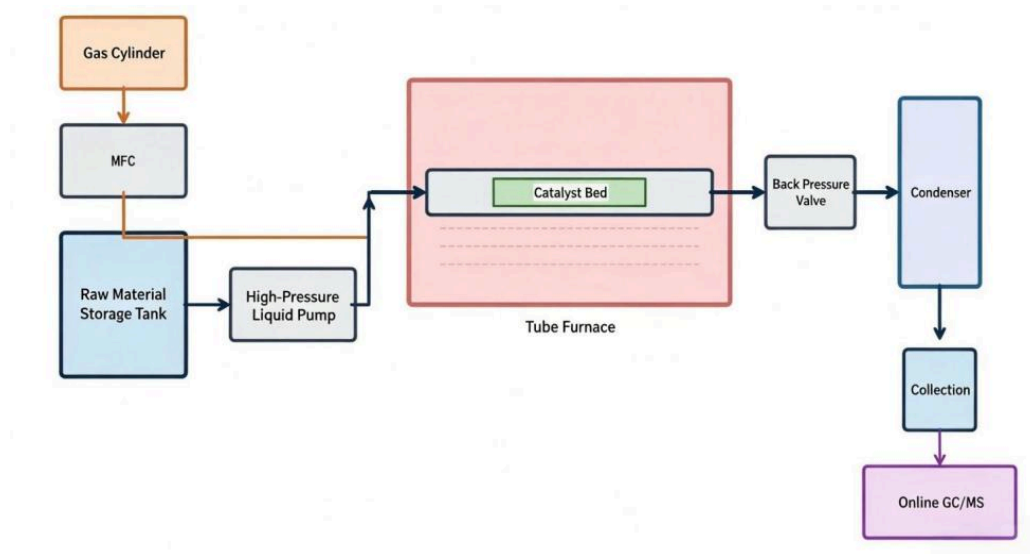
Figure 2. Schematic diagram of fixed-bed flow reactor
