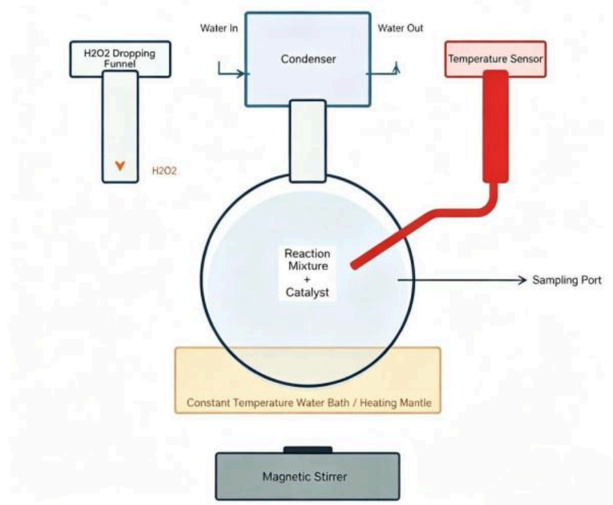
Figure 1. Schematic diagram of batch reactor
