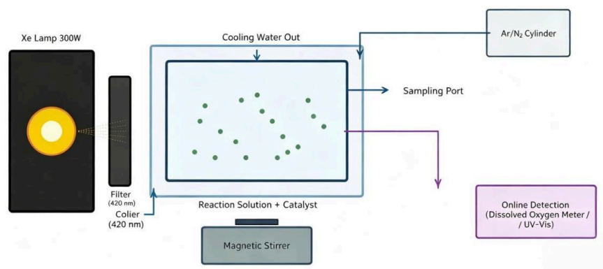
Figure 5. Schematic diagram of photocatalytic reactor
