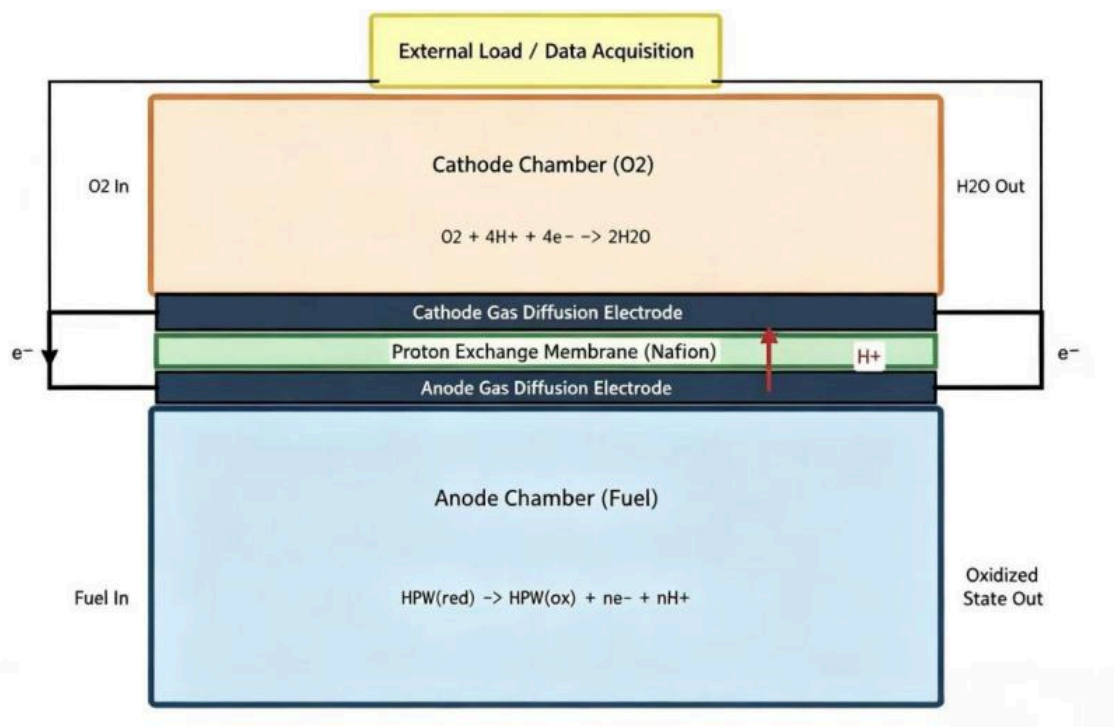
Figure 4. Schematic diagram of direct liquid fuel cell
