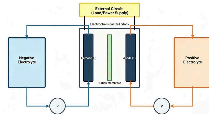
Figure 3. Schematic diagram of redox flow battery
