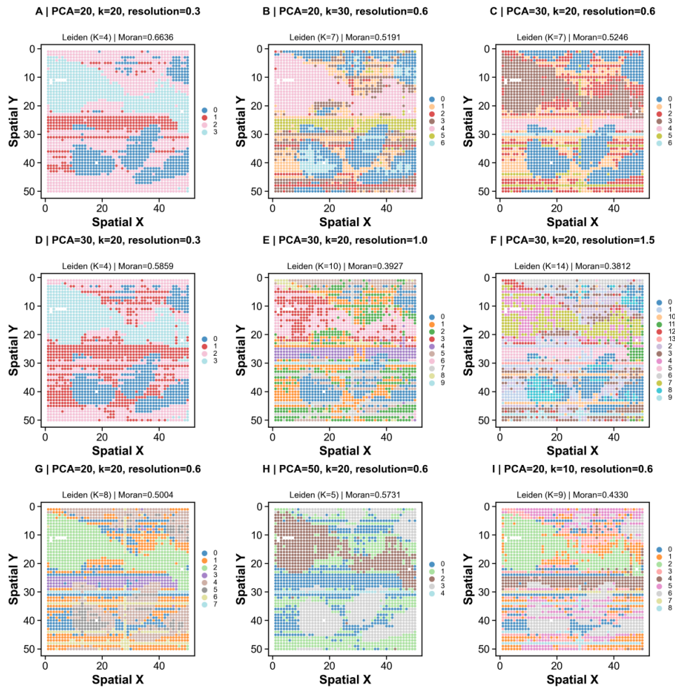
Figure 2. Parameter sensitivity of Leiden clustering on the HumanTonsil dataset. Based on gene-protein joint representations from 2 492 spatial spots, nine representative Leiden configurations (A-I) are presented. Panel A shows the configuration with maximum weighted Moran's I. Panels B-C produce seven clusters under different PCA-dimension and neighbour-number settings. Panels D-F demonstrate granularity shifts caused by resolution increments with fixed PCA dimension and k. Panels G-I further illustrate separate effects of PCA dimension, neighbour number and resolution. Each sub-panel labels the actual cluster count K and weighted Moran's I
