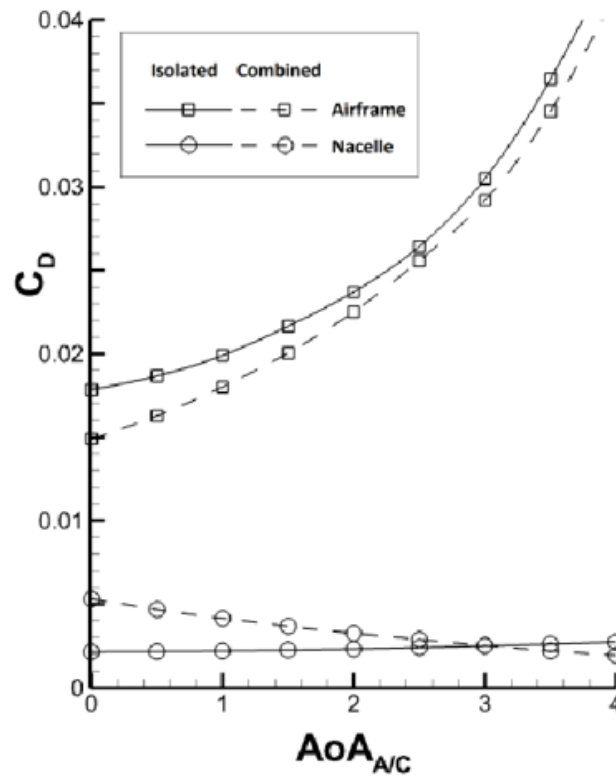
Figure 1. Aerodynamic drag trade-offs between airframe and nacelle configurations
