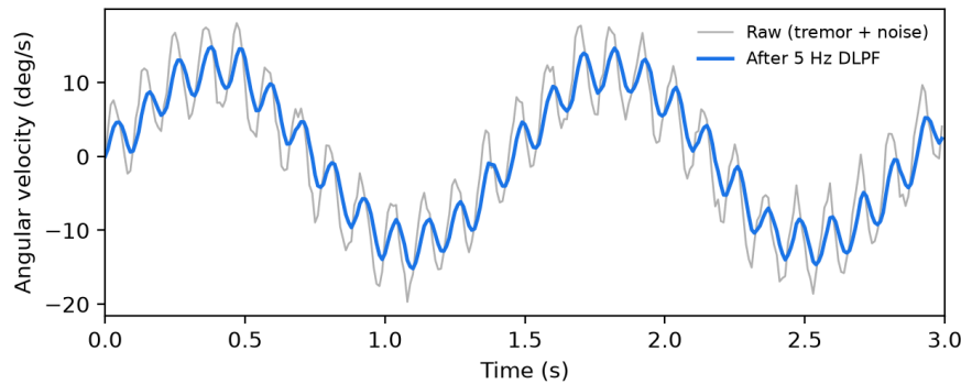
Figure 1. Angular-velocity waveforms: comparison of raw gyroscope signal (tremor + noise) and signal filtered via the 5-Hz MPU-6050 DLPF
