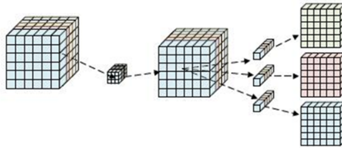
Figure 2. Schematic diagram of depth-separable convolution [6]
