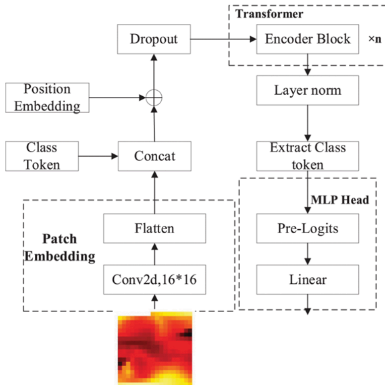
Figure 3. Overall framework of the ViT model [7]
