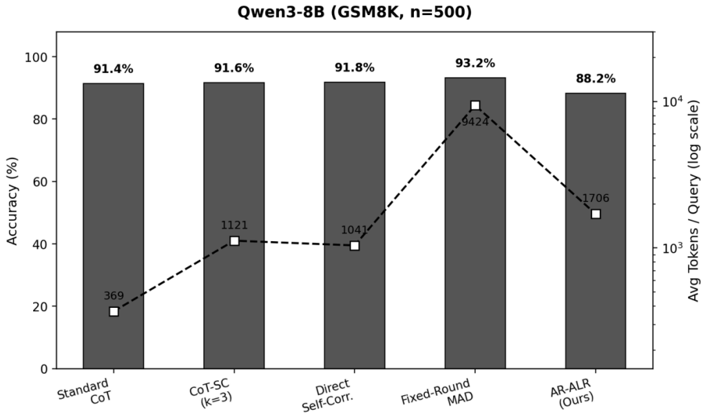
Figure 3. Comparison of accuracy and token cost across methods on Qwen3-8B (photo credit: original)
