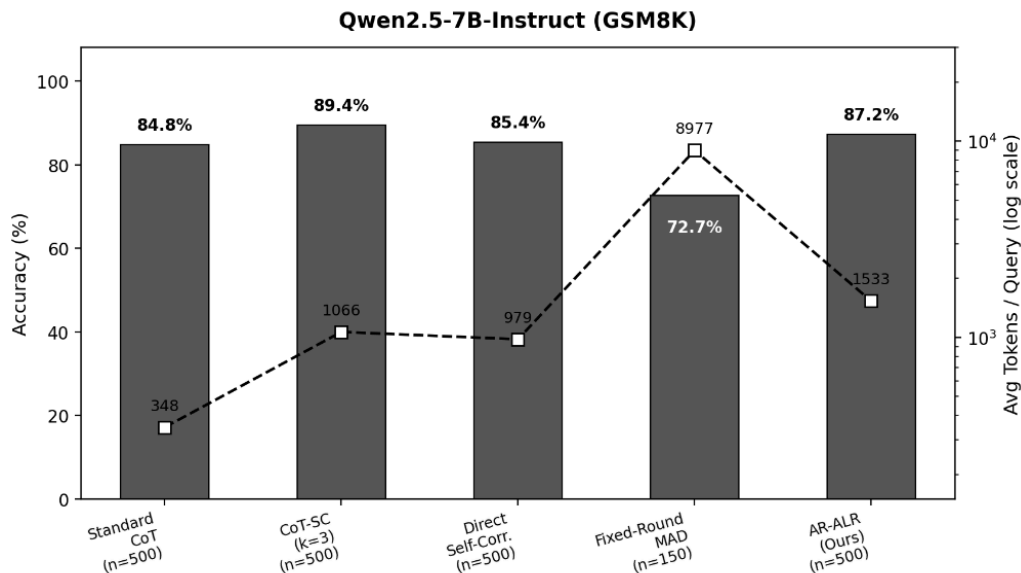
Figure 2. Comparison of accuracy and token cost across methods on Qwen2.5-7B-Instruct (photo credit: original)
