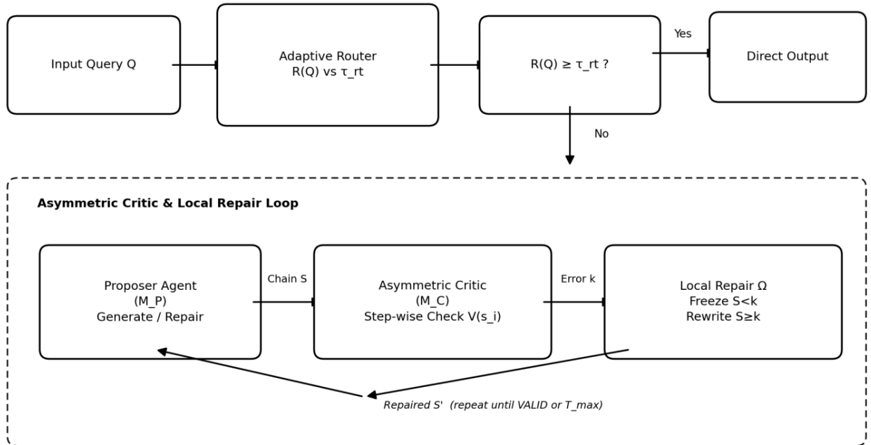
Figure 1. Overall architecture and data flow of the AR-ALR framework (photo credit: original)
