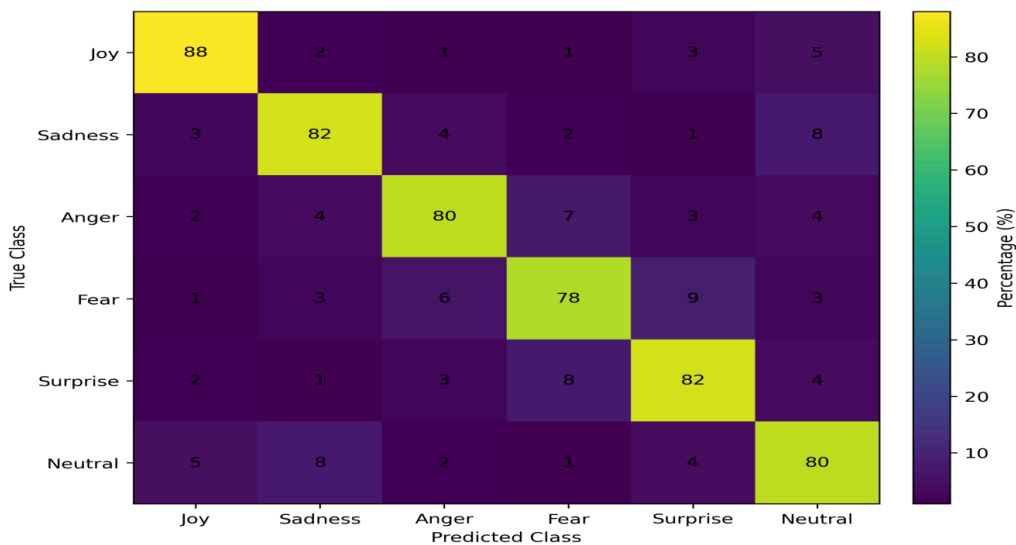
Figure 1. Normalized confusion matrix of six emotional categories for the trimodal model
