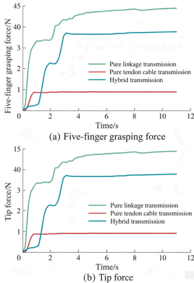
Figure 4. Comparative experimental curves of grip strength
