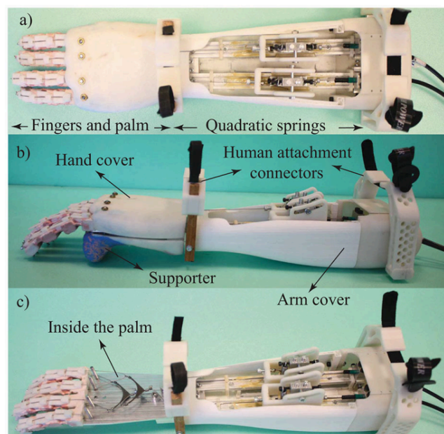
Figure 2. (a) Top view, (b) side view, and (c) interior of the transradial hand prosthesis prototype [5]
