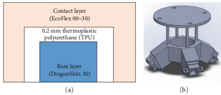
Figure 5. Design of the soft gripper. (a) Structural layers of finger design. (b) CAD model of finger mount [7]
