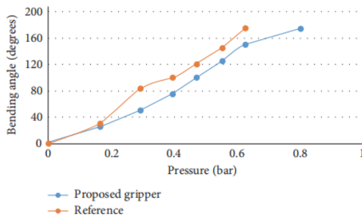
Figure 6. Comparative analysis of the bending angle for pressure difference [7]
