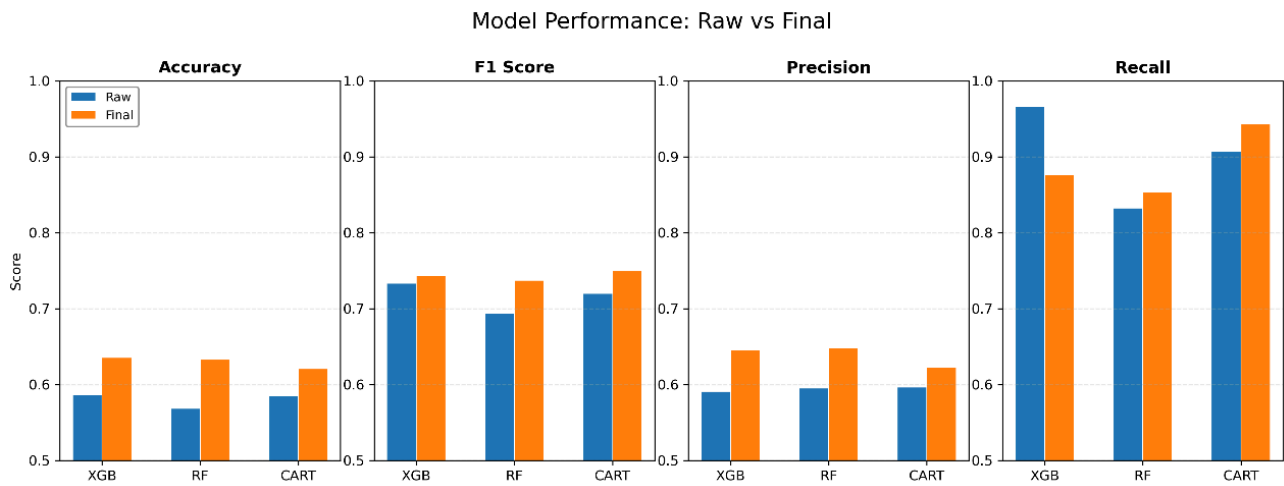
Figure 2. Model performance: raw vs final
