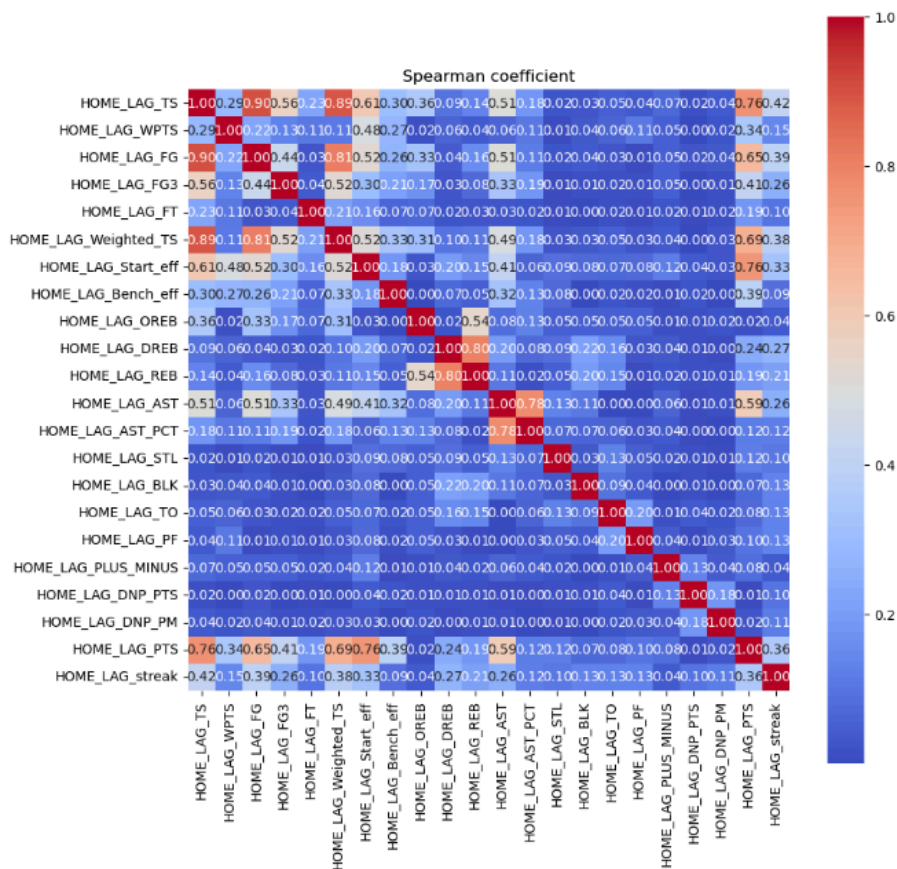
Figure 1. Heat map of the Spearman correlation
