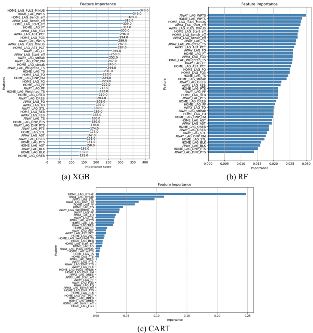
Figure 3. Feature importance of preprocessed data across three models
