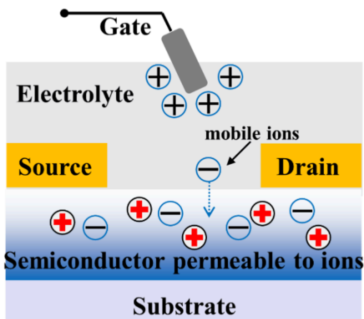
Figure 1. Schematic diagram of a typical vertical electrochemical transistor structure [3]
