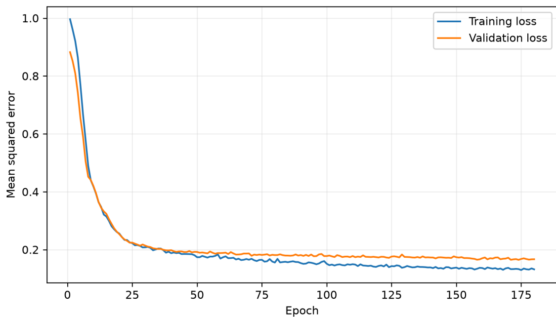
Figure 5. Training and validation loss of the proposed model for seed 42 (picture credit: original)
