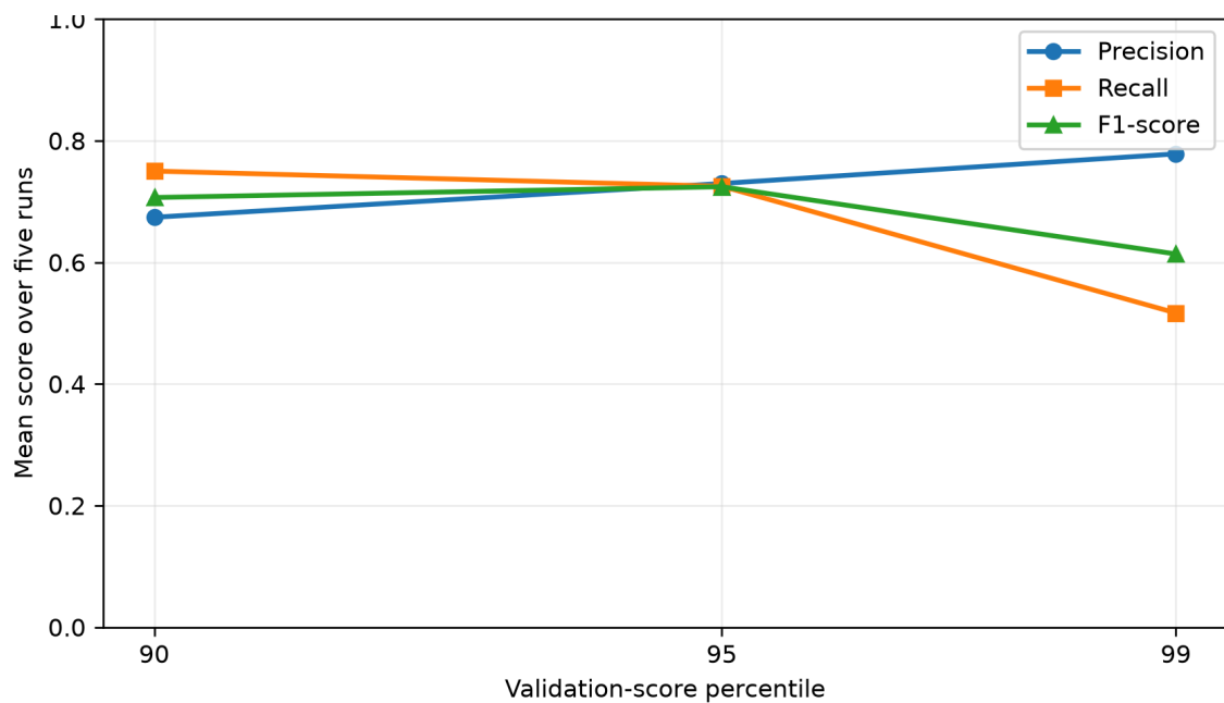
Figure 4. Precision, recall, and F1-score at three thresholds (picture credit: original)
