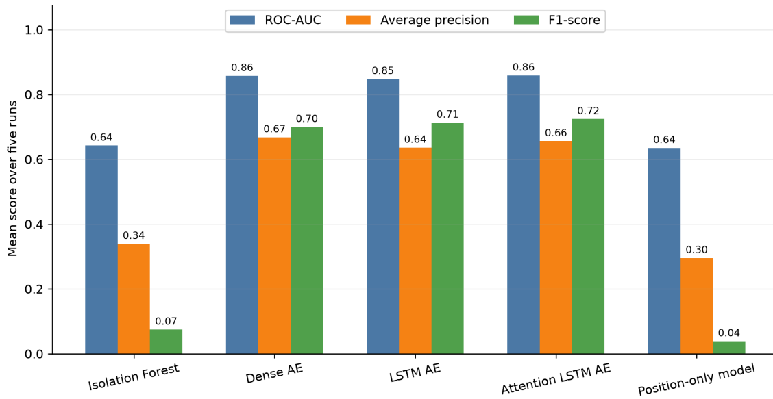
Figure 2. Performance comparison of the five anomaly detectors (picture credit: original)
