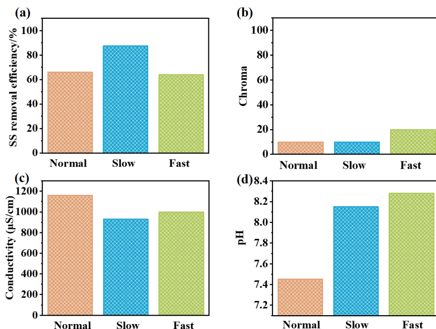
Figure 7. Effect of inflow rate on snowmelt water parameters: (a) SS, (b) color, (c) conductivity, and (d) pH
