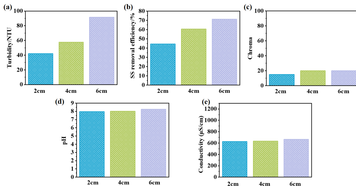
Figure 4. Effect of quartz sand filter bed thickness on snowmelt water parameters: (a) turbidity, (b) suspended solids (SS), (c) color, (d) pH, and (e) conductivity
