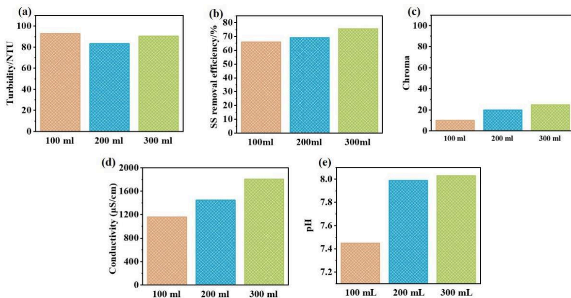
Figure 6. Effect of water volume on snowmelt water parameters: (a) turbidity, (b) suspended solids (SS), (c) color, (d) conductivity, and (e) pH
