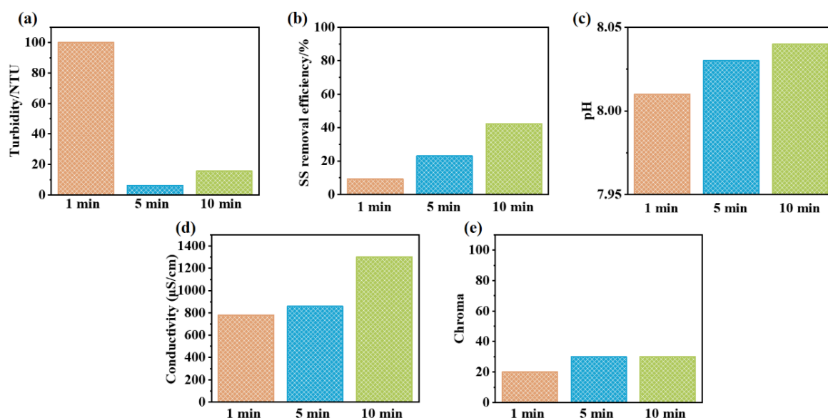
Figure 5. Effect of filtration time on snowmelt water parameters: (a) turbidity, (b) suspended solids (SS), (c) pH, (d) conductivity, and (e) color
