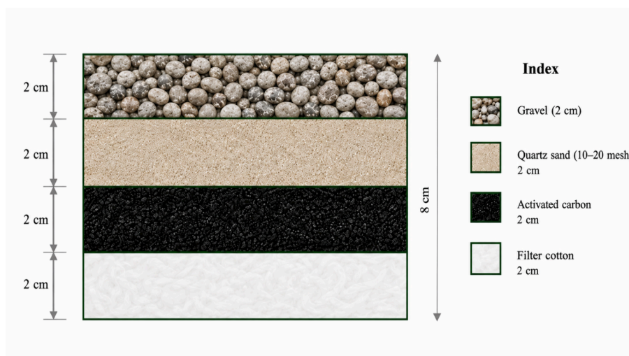
Figure 2. Schematic cross-sectional view of a standard filtration unit (filter cotton: FC, activated carbon: AC, quartz sand: QS, and gravel: GR)
