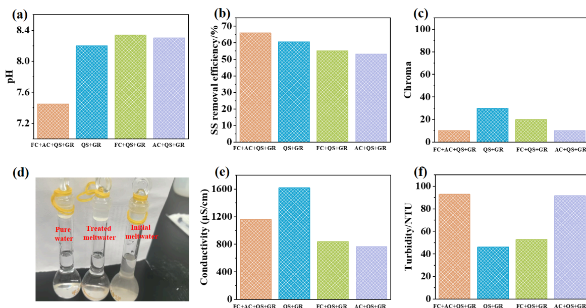
Figure 3. Effects of different filter media combinations(filter cotton: FC, activated carbon: AC, quartz sand: QS, and gravel: GR) on snowmelt water parameters: (a) pH, (b) suspended solids (SS), (c) color, (d) hue, (e) conductivity, and (f) turbidity
