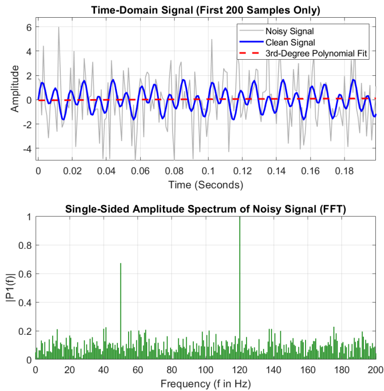
Figure 3. Single-sided amplitude spectrum of the noisy signal (picture credit: original)
