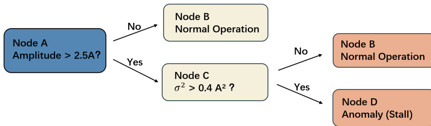
Figure 4. Random Forest Classifier (picture credit: original)
