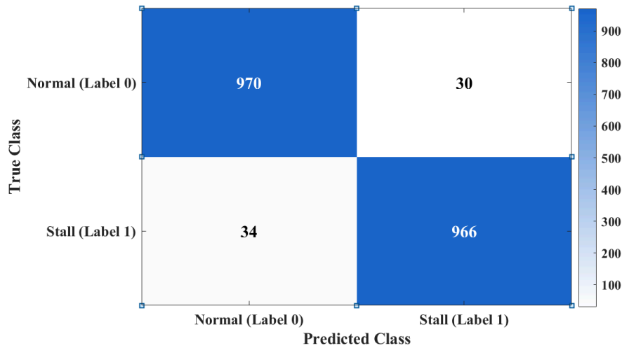
Figure 5. Confusion matrix of random forest classifier (picture credit: original)
