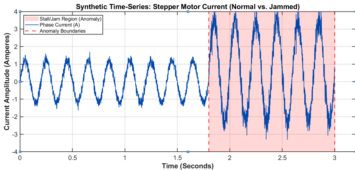
Figure 1. Synthetic time-series of the stepper motor phase current (picture credit: original)
