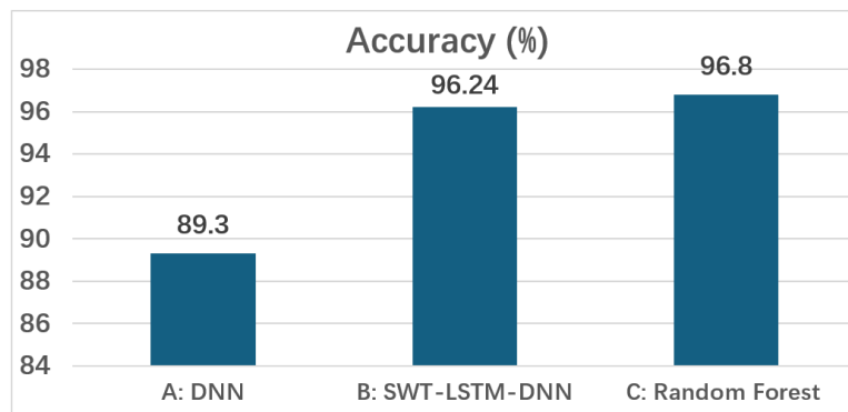
Figure 6. Accuracy comparison of anomaly detection algorithms (picture credit: original)
