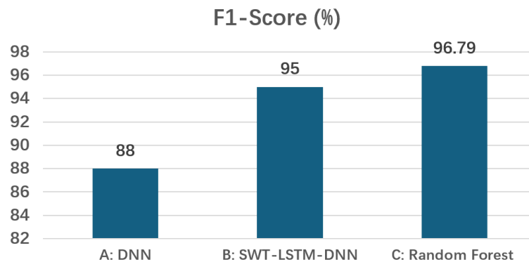
Figure 7. F1-Score comparison of anomaly detection algorithms (picture credit: original)
