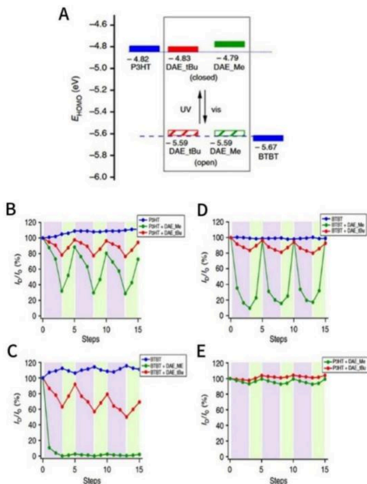
Figure 7. (A) Energy level diagram illustrating HOMO alignment between semiconductors and DAEs in open/closed forms. (B–E) Reversible photoswitching cycles of normalized drain current under UV (365 nm) and visible (546 nm) light [23]
