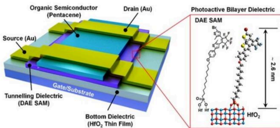
Figure 5. Schematic cross section of a PHBD OMT
