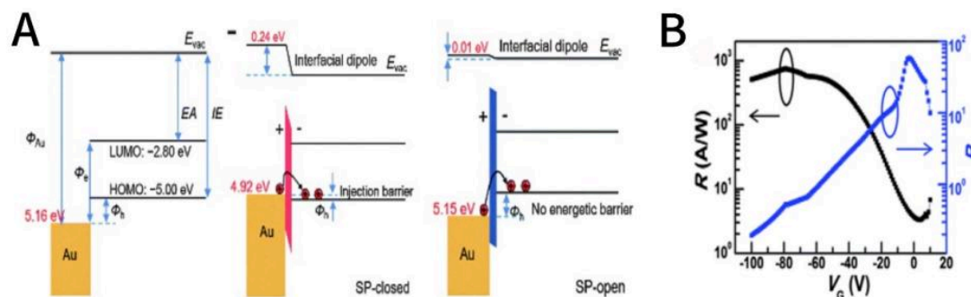
Figure 4. (A) Energy level diagrams of working function of Au ( \Phi_{Au} ), HOMO and LUMO energy levels of pentacene, pristine injection barrier of electrons ( \Phi_e ) and holes ( \Phi_h ). (B) Responsivity (R)-gate voltage curve and photosensitivity (P)-gate voltage curve ( V_D = -100 V). Effective irradiance power: 7.4 mW cm -2 [17]
