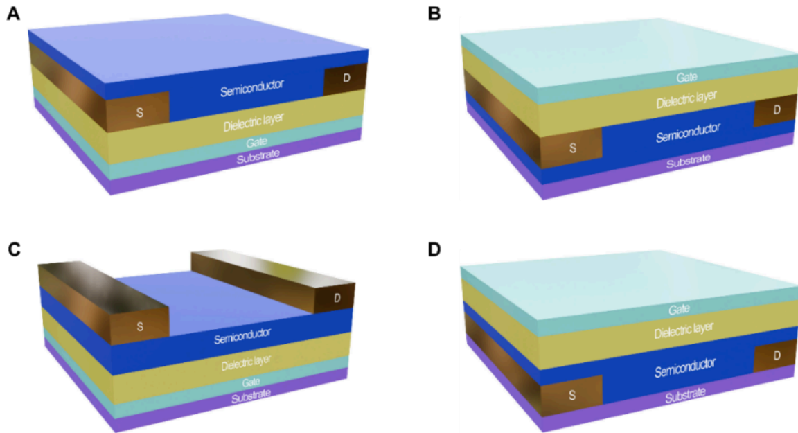
Figure 1. Different architectures of OFETs. (A) bottom contact and bottom gate. (B) bottom contact and top gate. (C) top contact and bottom gate. (D) top contact and top gate
