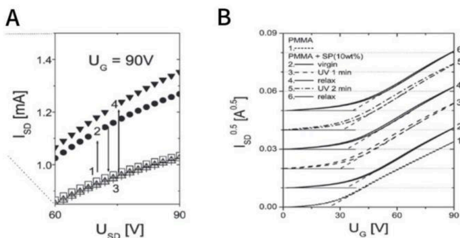
Figure 6. (A) U_G = 90 V showing the switching cycle. (B) Locus ( U_{SD} = U_G ) current-voltage characteristics for PMMA/P13 (curve 1) and (PMMA + SP)(10 wt %)/P13 FETs (curves 2-6)
