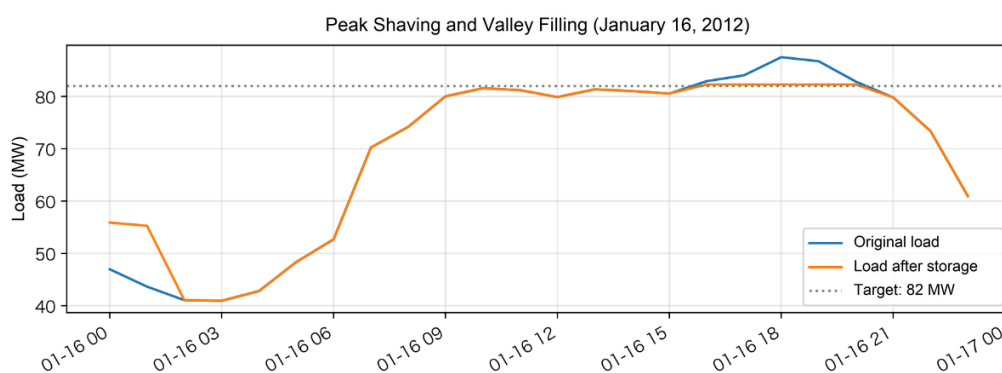
Figure 3. Peak shaving and valley filling on January 16, 2012 (picture credit: original)
