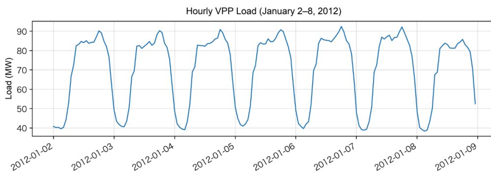
Figure 1. Hourly load of the VPP portfolio, January 2–8, 2012 (picture credit: original)
