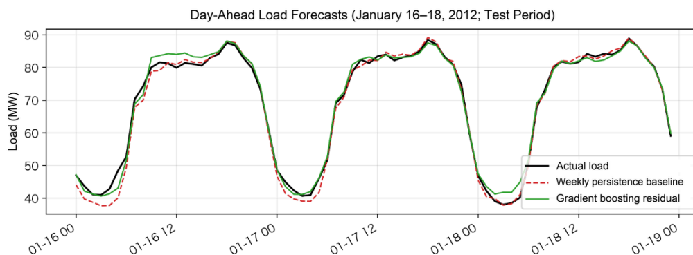
Figure 2. Day-ahead load forecasts, January 16–18, 2012 (picture credit : original)
