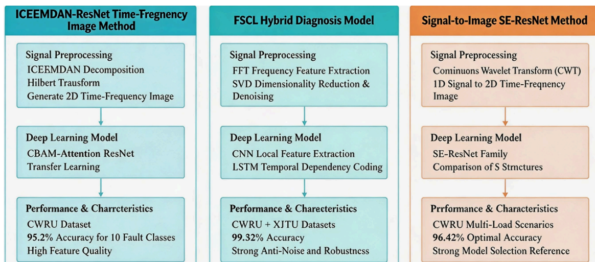
Figure 1. Core architecture of three representative deep learning fault diagnosis methods for rolling bearings (picture credit: original)
