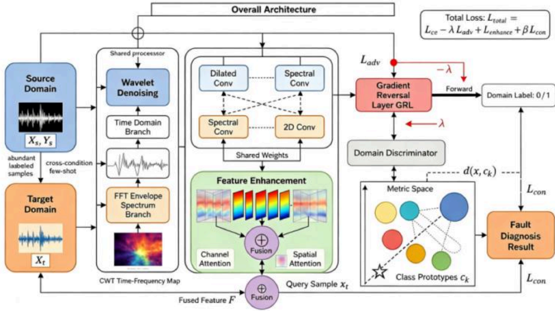
Figure 1. Overall architecture of the Feature-Enhanced Fusion and Adversarial Domain Adaptation (FEF-ADA) model
