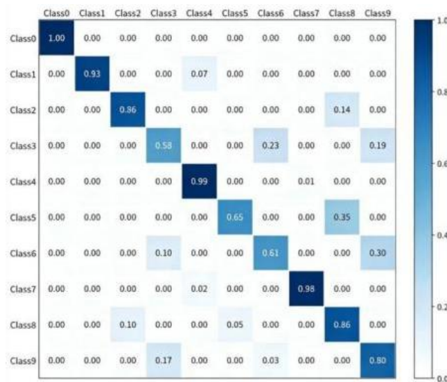
Figure 3. Confusion matrix
