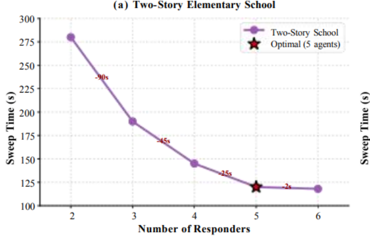
Figure 5. Responder scaling analysis. (a) School optimal at 5 agents. (b) Warehouse optimal at 4 agents. Marginal gains negligible beyond these points
