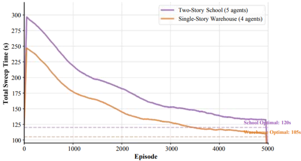
Figure 4. Training convergence comparison. Warehouse converges faster through horizontal partitioning; school demands extended exploration for multi-floor strategies
