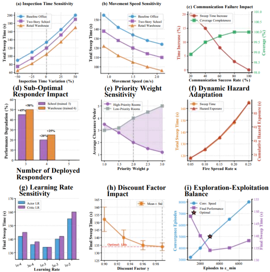
Figure 6. Comprehensive sensitivity analysis across environmental parameters (top row), coordination mechanisms (middle row), and training hyperparameters (bottom row)
