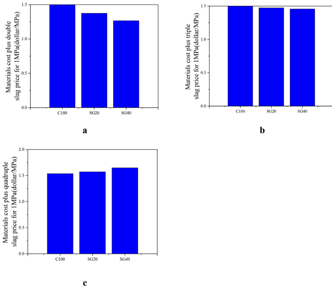
Figure 1. The impact of rising slag prices on the unit strength material cost of concrete: (a) doubled slag prices, (b) tripled slag prices, (c) quadrupled slag prices [15]
