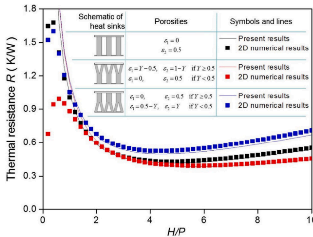
Figure 3. Schematic illustrating the effect of height variation on thermal resistance under different shapes [12]
