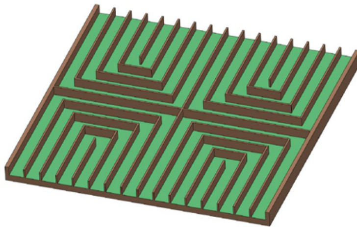
Figure 1. Schematic of a four-quadrant microchannel heat sink [3]
