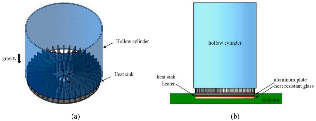
Figure 2. (a) Radiator geometry; (b) Experimental setup [8]
